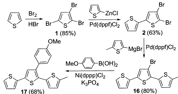
Scheme 1. Sequential regioselective couplings.
